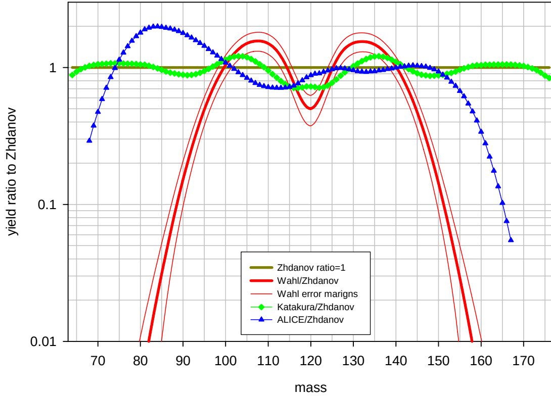
Benchmark B: ^{244}\text{Cm} at 28 MeV, post neutron emission yield ratios to Zhdanov's data
